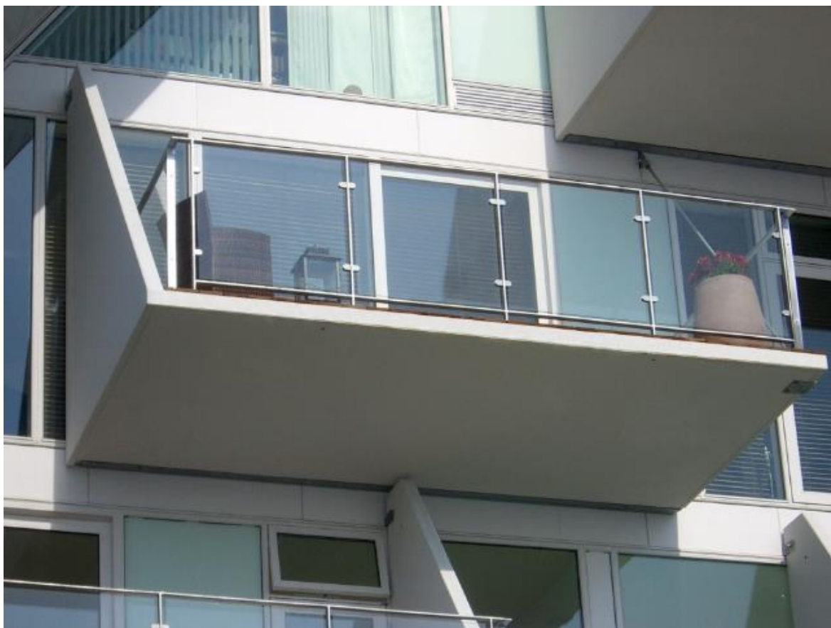
Fig. 6 Balcony combining concrete upstand and strut.
